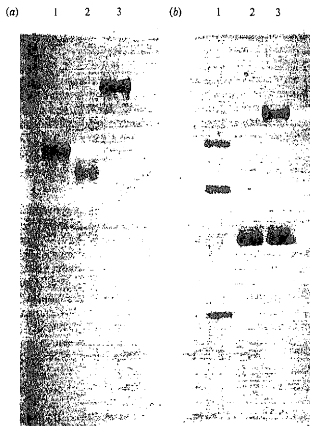
Fig. 1. Polypeptide compositions of haemagglutinin and HA 'tops'. Bromelain-released haemagglutinin (BHA) and the HA 'tops' and aggregate fractions obtained by tryptic digestion of BHA in the pH 5.0 conformation were purified as described in Methods. Samples were boiled in either 0.5% SDS and 8 M-urea or 0.5% SDS, 8 M-urea and 0.05 M-2-mercaptoethanol for 2 min before electrophoresis on polyacrylamide gels containing 16.5% acrylamide for 16 h at 10 V/cm as described previously (Skehel et al. , 1982). (a) Lane 1, HA 'tops'; lane 2, aggregate; lane 3, BHA, non-reduced samples. (b) Lane 1, HA 'tops'; lane 2, aggregate; lane 3, BHA, reduced samples.
