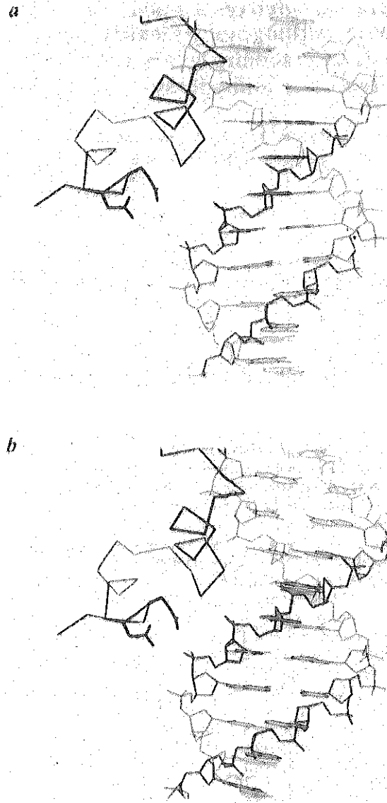
Fig. 3 Interaction of Asn 16 and Gln 17 with straight and bent DNA showing the \alpha -carbon backbone of \lambda -repressor residues 30-60 (ref. 13), positioned as described by Anderson et al. 1 , with the side chains of Asn 16 and Gln 17 of 434 repressor extending toward the DNA. In a , straight B-DNA was constructed by extending the double helix of the model DNA that best fits the electron density of one 14-bp operator 1 . The amino nitrogens of the Asn 16 and Gln 17 side chains are both >5 \text{ \AA} from the oxygens of the -1 phosphate, which is too far for hydrogen-bond formation. In b , B-DNA with a slight right-handed supertwist, generated as described by Anderson et al. 1 , was positioned so that 14 bp of the modelled DNA gave the best fit to the electron density of one 14-bp operator. The side-chain amino groups of Asn 16 and Gln 17 are separated from the phosphate oxygens by \sim 3 \text{ \AA} , a typical hydrogen-bond length.
