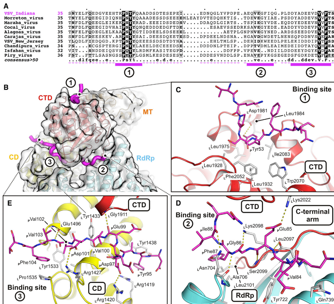
Figure 2. Molecular Details of Phosphoprotein Interactions with the L Protein
