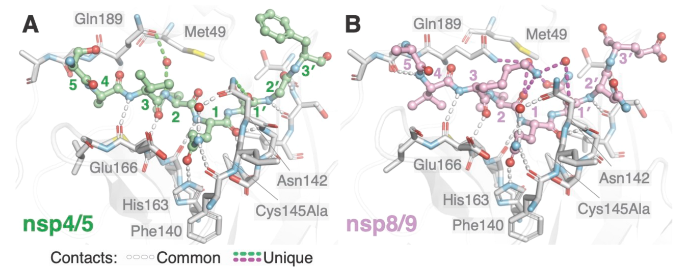
Figure 2. Differential recognition of nsp4/5 and nsp8/9 substrates by M Pro . Identical views of nsp4/5 (A) and nsp8/9 (B) substrates in the M Pro Cys145Ala active site. Substrate peptide P and P' residues are labeled with colored numbers. Key M Pro residues mentioned in the text are labeled. Conserved hydrogen bonds enabling M Pro recognition of substrate mainchain and P1 Gln side chain atoms are shown as white dashed lines. Hydrogen bonds that differ between the complex with nsp4/5 and that with nsp8/9 are shown in green and magenta, respectively. M Pro Asn142 and Gln189 contact both substrates through bound water molecules, and the resulting networks of hydrogen bonds differ between the two substrates.
